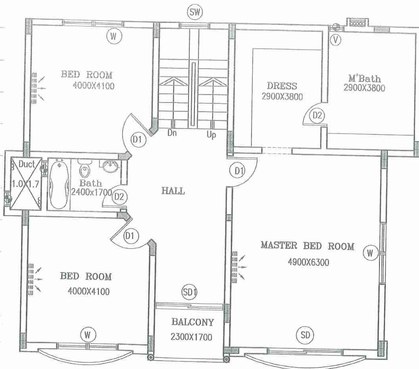
First Floor Plan Villa-2 B.U.Area:131.00 Sqmts
