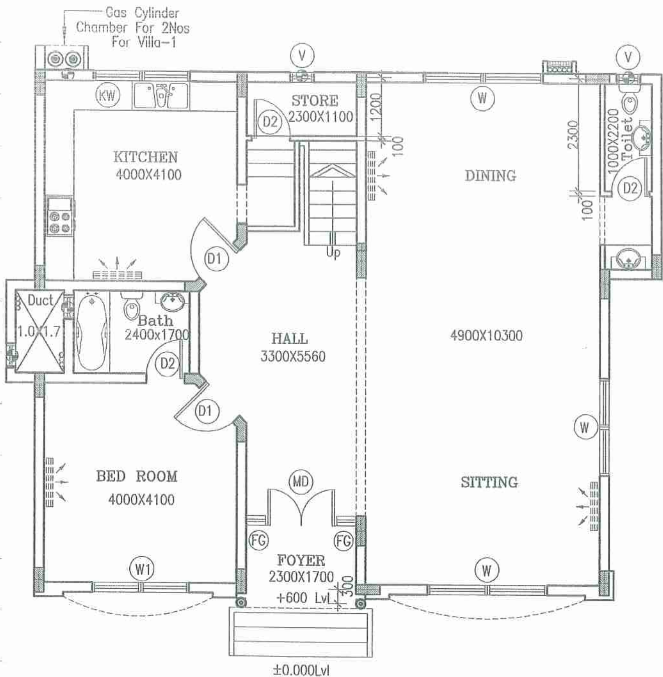
Ground Floor Plan Villa-2 B.U.Area:131.00 Sqmts
